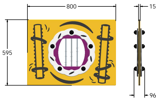
FIDANDSC6 FIDANDSC6-AL-WP Standard Panel Panel with Alu Posts
