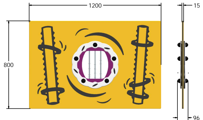
FIDANDSC3 FIDANDSC3-AL-WP Standard Panel Panel with Alu Posts
