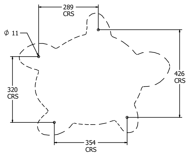
Host Panel Fixing Detail
