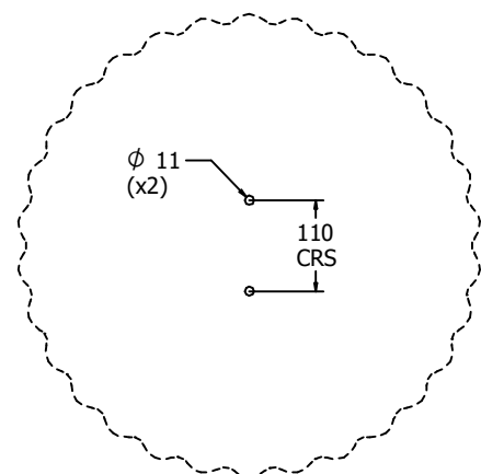
Required Host Panel Fixing Detail
