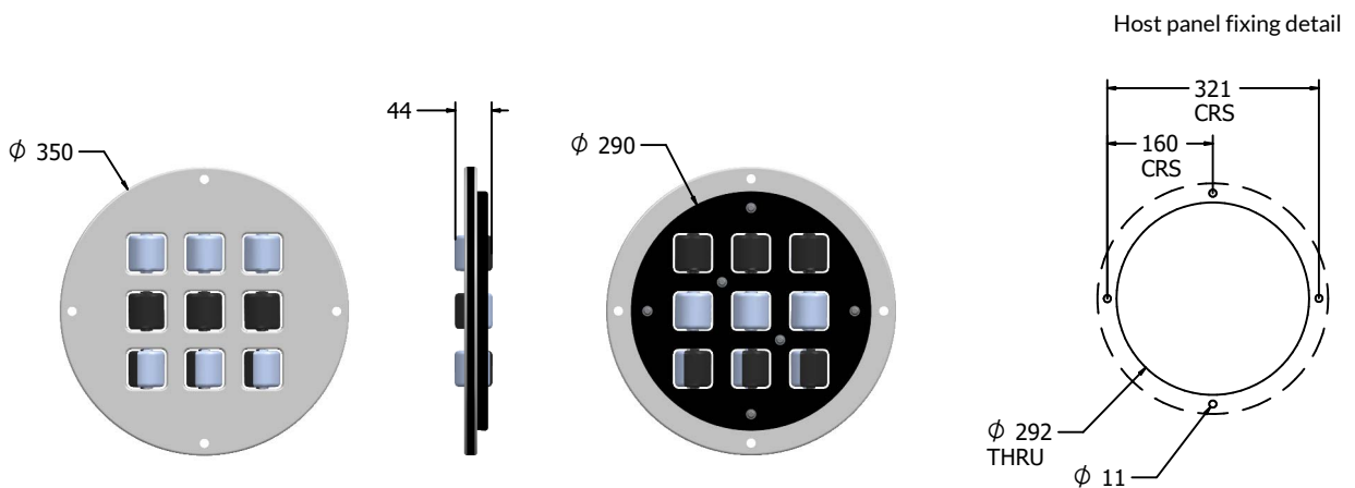
Insert can be easily attached to your own panel
