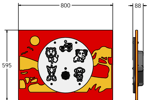
FIPTSSAFA6 Standard Panel
