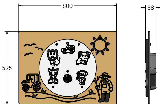
FIPTSFARM6 Standard Panel FIPTSFARM6-AL-WP Panel with Alu Posts
