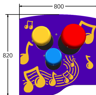
FIMUBON3 - Standard Panel FIMUBON3-AL-WP - Panel with Alu Posts
