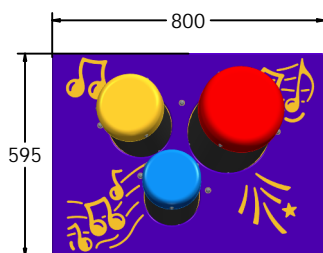
FIMUBON6 - Standard Panel FIMUBON6-AL-WP - Panel with Alu Posts
